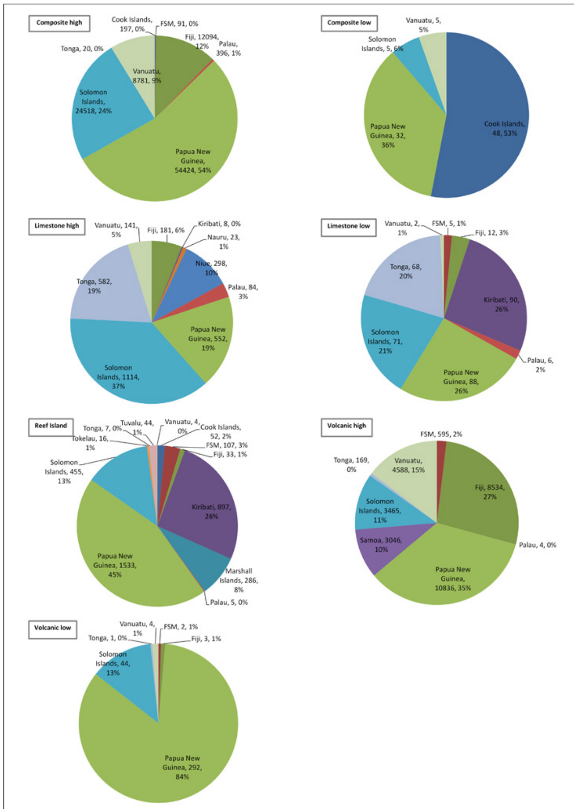
Figure 2.6 Detailed breakdown for each Pacific Island country of each island type by area and the proportion found in each country. The numbers give the total area (km 2 ) and the percentage of that area in the particular category.
