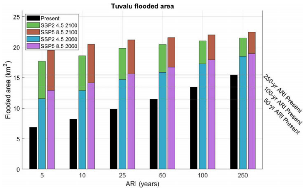
Figure 9-9 Flooded area (km 2 ) above MHWS across all of Tuvalu for different annual return intervals (ARIs) and sea levels. Colours represent different sea level scenarios. 50-yr ARI, 100-yr ARI, and 250-yr ARI under present sea levels are highlighted by grey lines for comparison. Source: Wandres et al., 2024
